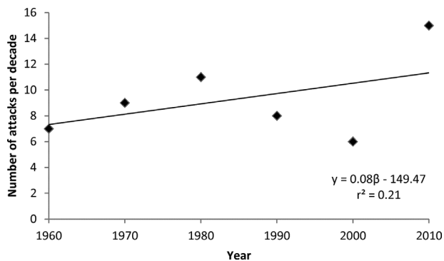
Figure 4. Number of polar bear attacks on humans by decade (e.g., 1960–1969) from 1960–2014.
